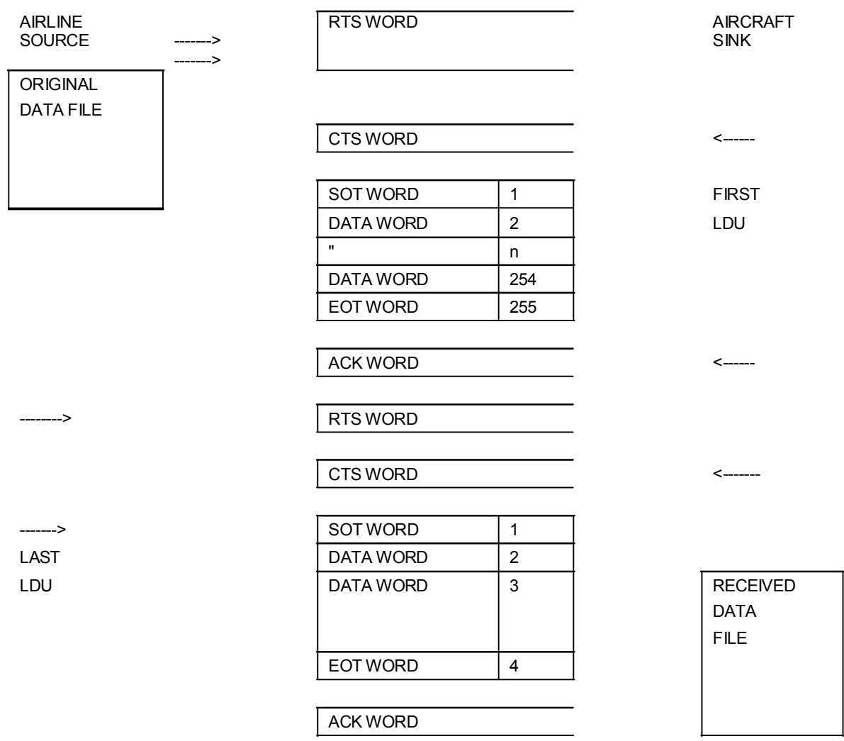
Figure 8. File Transfer Scheme Version 1 (no Windows)
