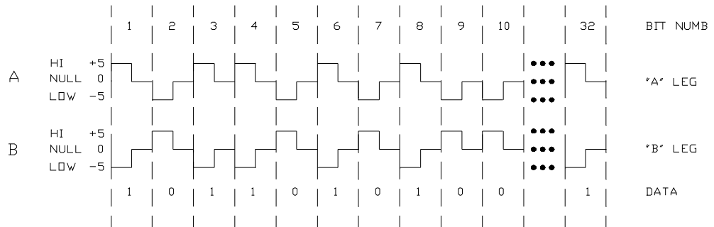
Figure 1. ARINC 429 Bit Encoding Example
